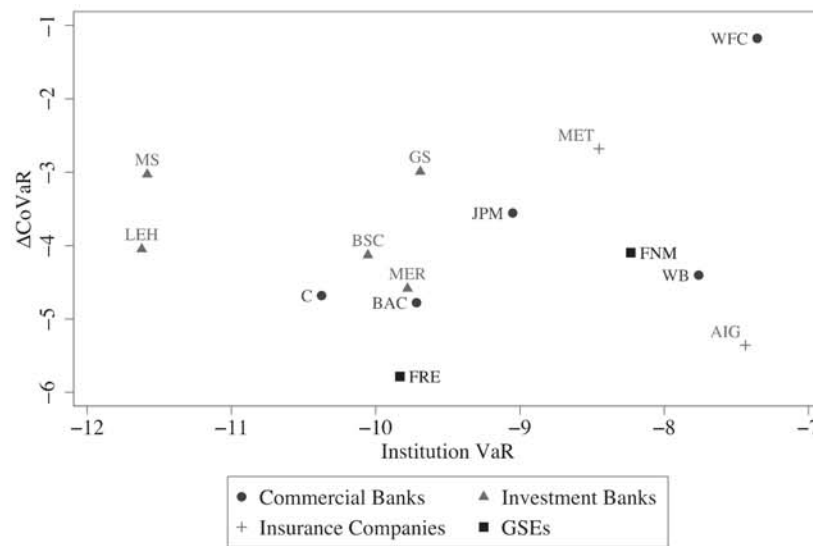
FIGURE 4: COVaR vs. VaR
